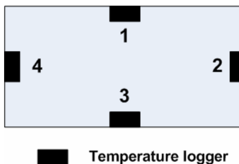
Figure 3 Possible locations inside a case (top view)
